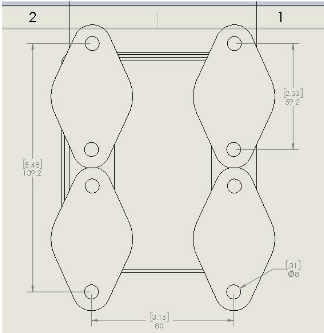
Figure 7: Feed Pump Assembly Foot Mount Drawing
