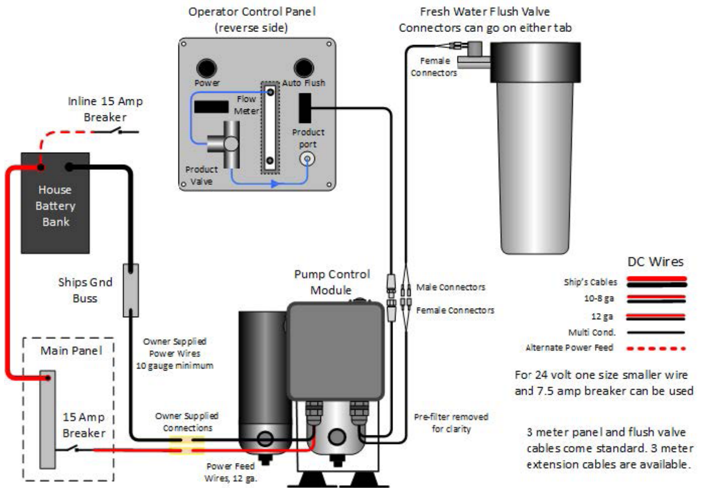
Figure 22: Electrical Diagram
