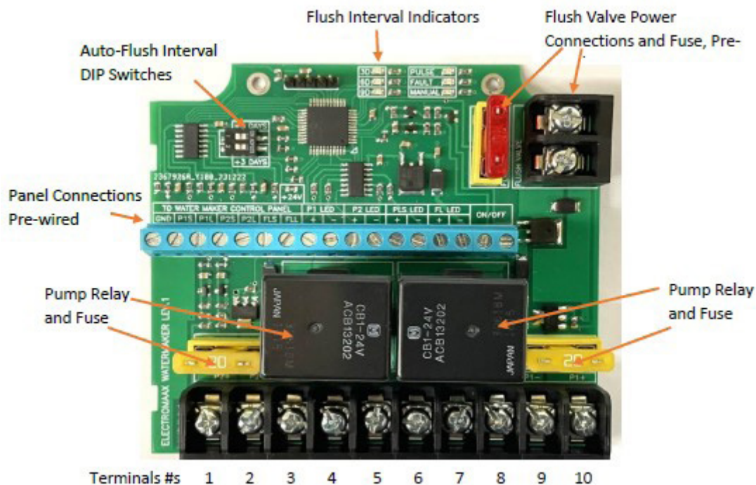
Figure 24: Pump Control Circuit Board
