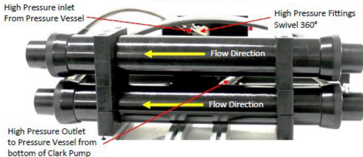
Figure 11: Rear View
