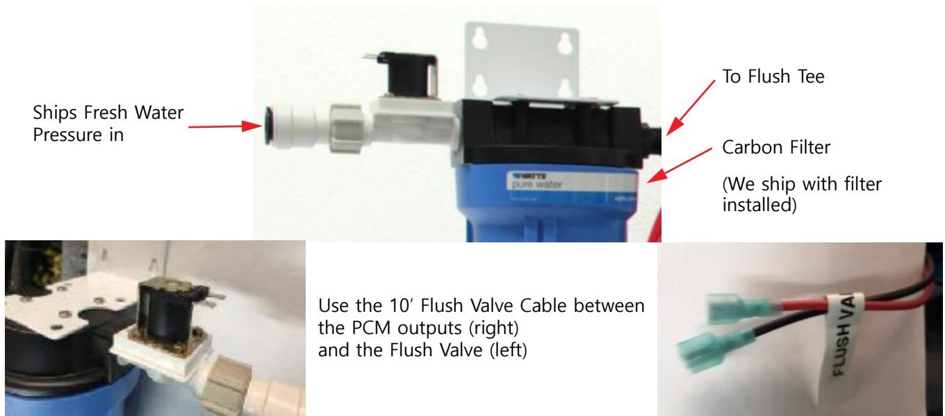
Figure 4: Freshwater Flush Assembly
