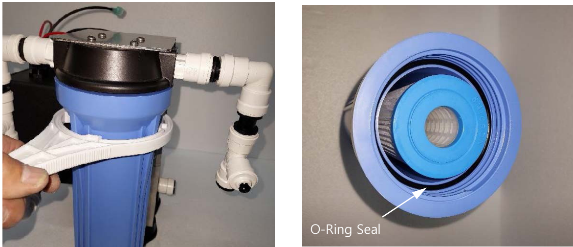
Figure 27: Micron Pre-Filter
