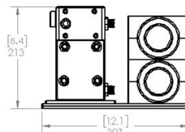
Figure 3: High Pressure Module Duel 21" Membrane Dimensions and Weight
