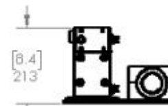
Figure 37: High Pressure Module 40" Membrane Dimensions and Weight
