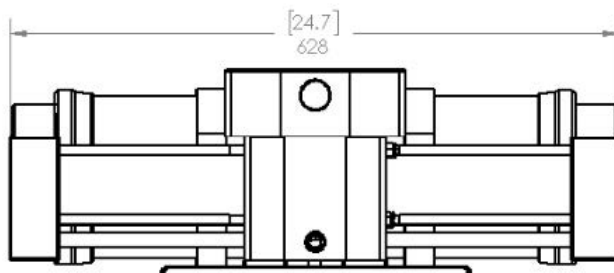
Figure 3: High Pressure Module Duel 21" Membrane Dimensions and Weight
