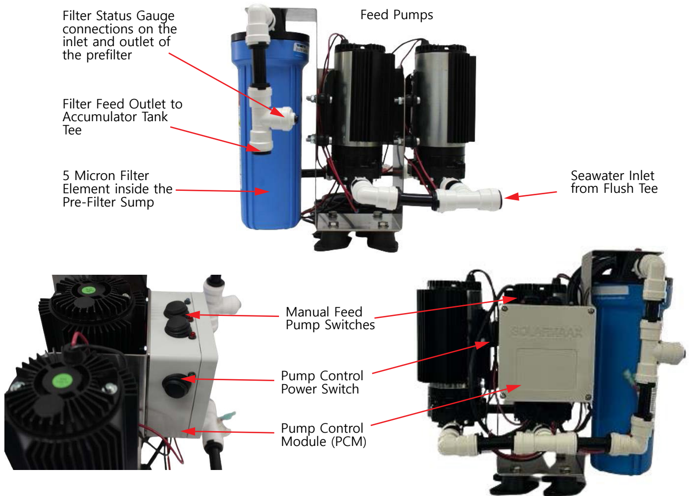
Figure 6: Feed Pump Assembly
