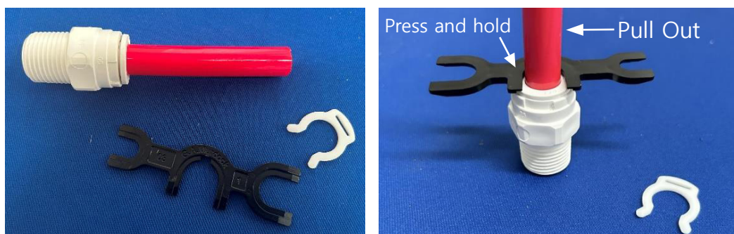
Figure 21: Tubing Removal Assist Tool
