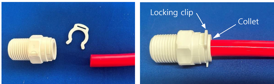
Figure 20: Fitting, Locking Clip & Tubing Installation
